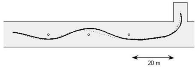
Figure 7: Trailer maneuver with slalom and parking driven by an experienced driver. The solid line is with linearised \gamma -controller and the dashed line is without controller
