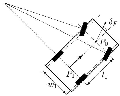
Figure 1: The Ackermann steering geometry.
